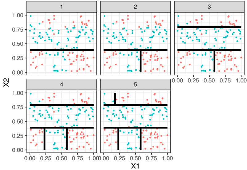
Figure 8.2 – Exemple de coupures successives.
