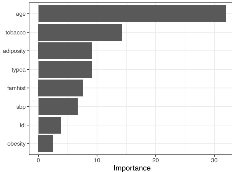
Figure 8.16 – Importance des variables.
